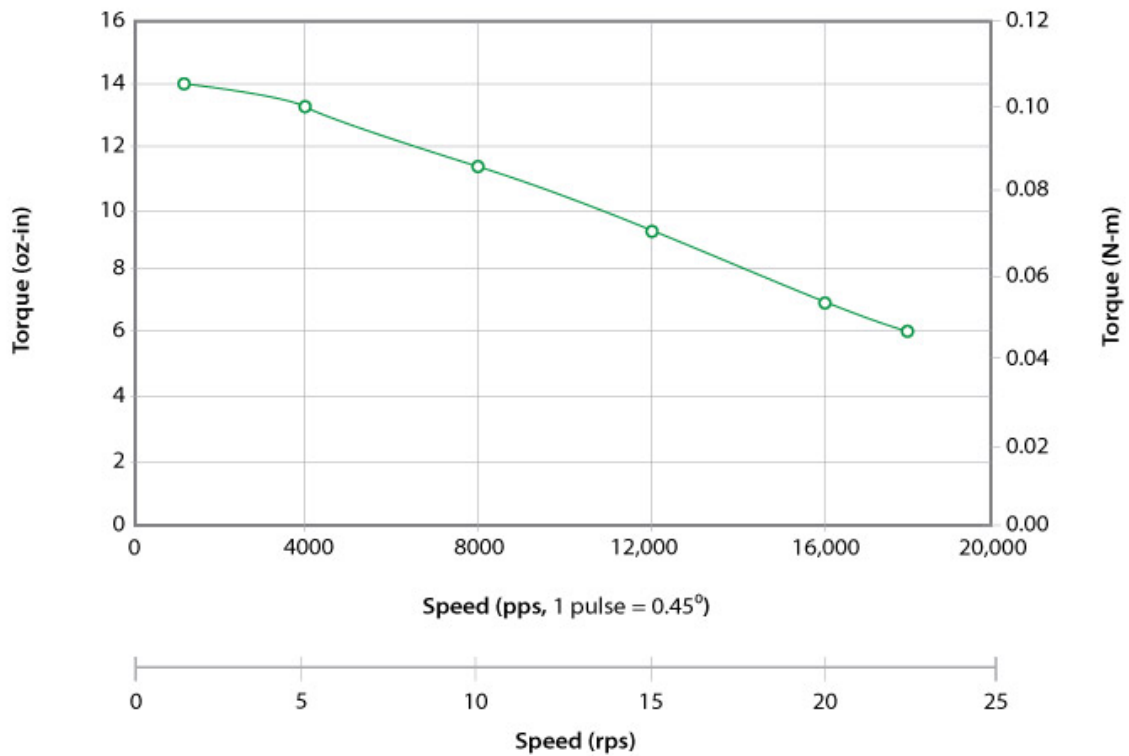
4109V-51 24VDC, 1.2 Amps/Phase, Bipolar, 1/2 Stepping
